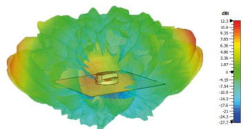
Typical 3D Pattern - WiFi Elements 5400MHz
