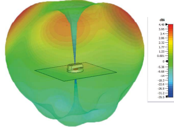
Typical 3D Pattern - 4G/5G Elements 1800MHz
